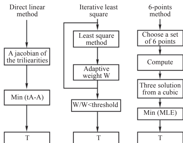
Fig. 3. Methods of estimation of the trifocal tensor.
