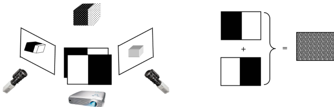
Fig. 1. Principle of imperceptible structured light. (Left) Trinocular sensor based on imperceptible structured light. The pattern is visible from one camera but not from the other and nor from human eye. (Right) Integration over time of the initial pattern and its complement due to high frequency projection.
