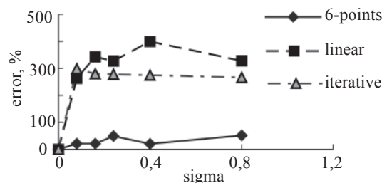
Fig. 4. Left: distance between intersection of epipolar lines and real point. Right: Difference between real points and transferred points, estimated by the transfer relation.
