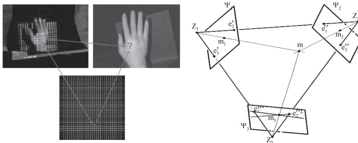
Fig. 2. Left: the correspondence problem. Right: Trifocal geometry, e are the epipoles, Z the projection centre and \Psi the image planes.
