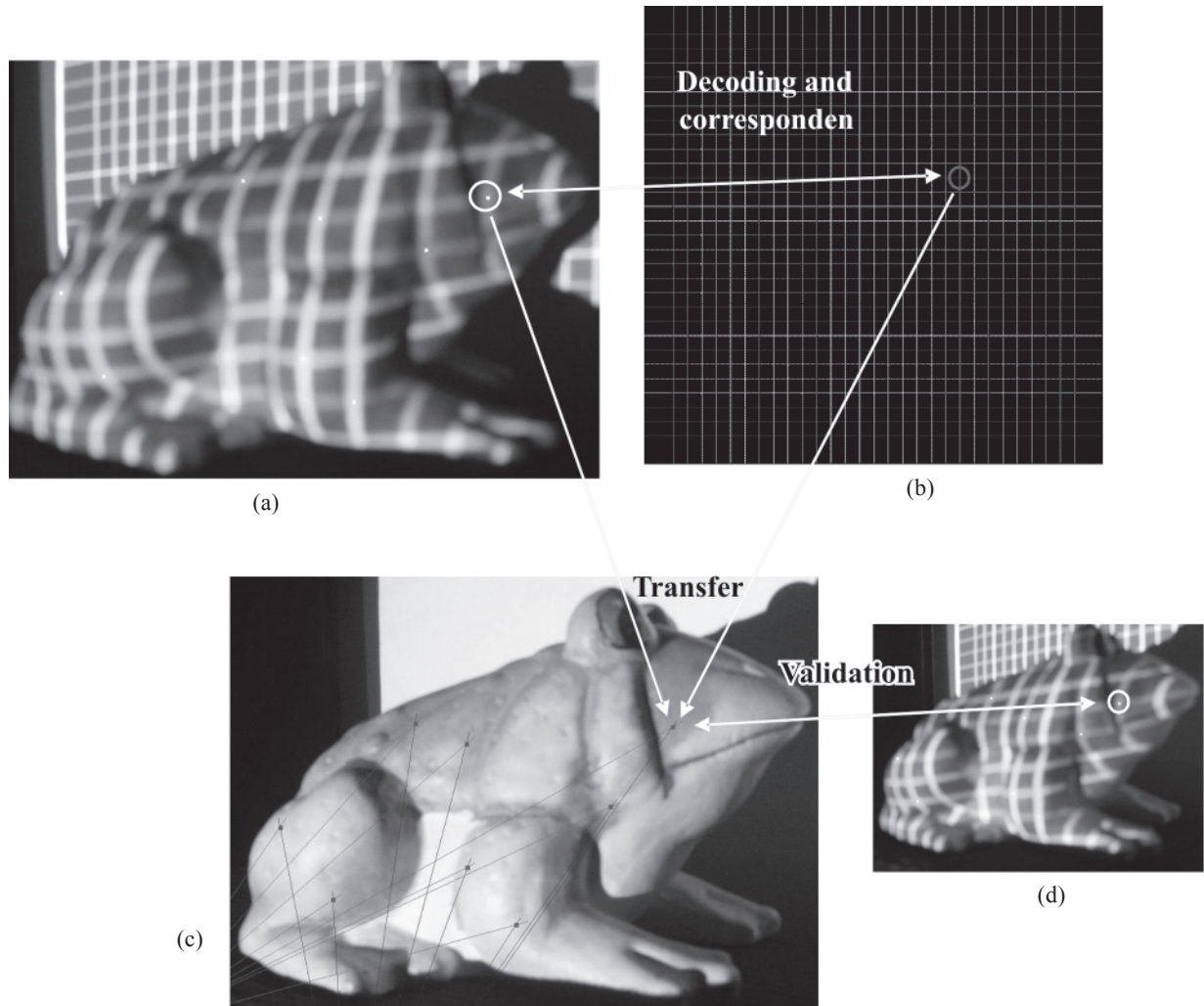
Fig. 5. (a) View as perceives by camera 1. (b) Initial projected pattern. (c) Transferred points in view 2. (d) View 2 with projector switched on so as to validate the transfer: transferred point lies exactly on the good code.
